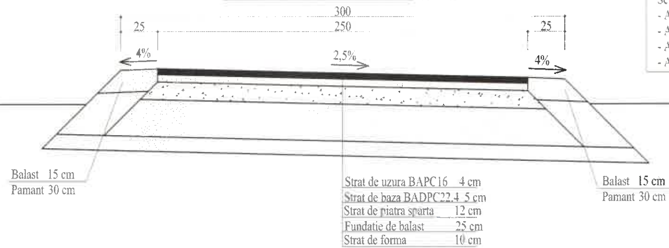
PROFIL TRANSVERSAL CARACTERISTIC TIP 2
