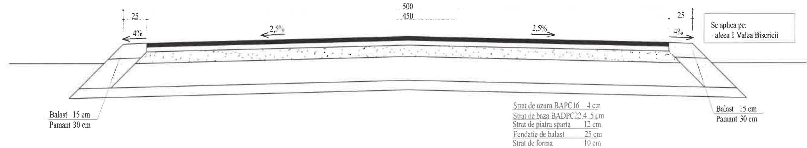
PROFIL TRANSVERSAL CARACTERISTIC TIP 1
